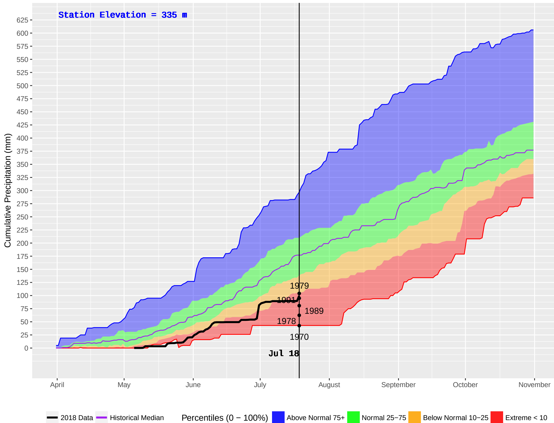
KISPIOX HUB (428) : Historical (1970–2016) and Current (2018) Daily Cumulative Precipitation
