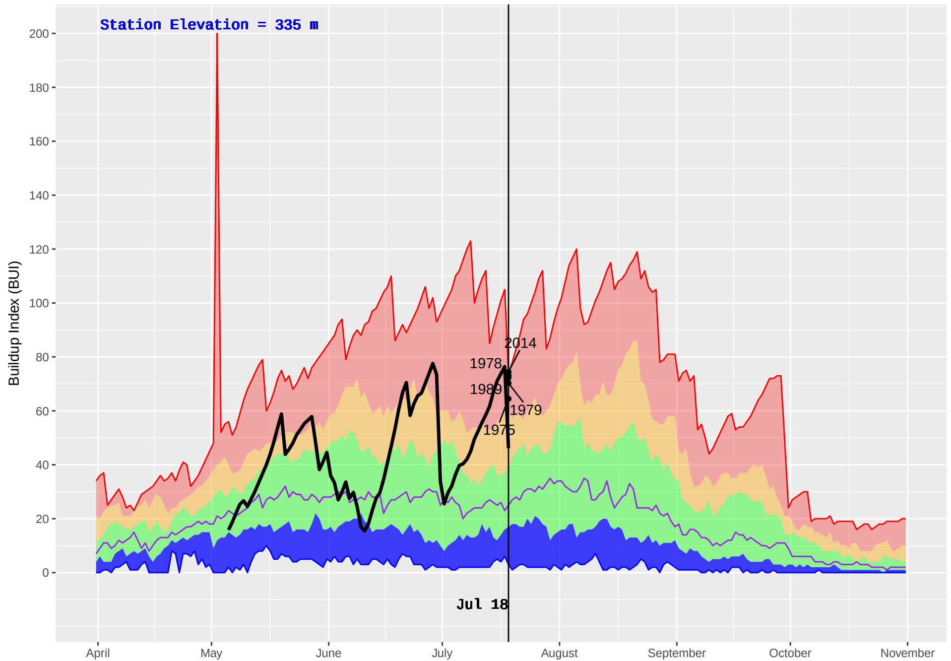
KISPIOX HUB (428) : Historical (1970–2016) and Current (2018) Daily Buildup Index (BUI)
