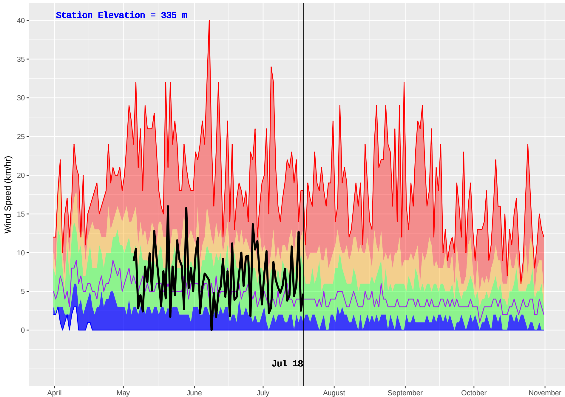
KISPIOX HUB (428) : Historical (1970–2016) and Current (2018) Daily Wind Speed
